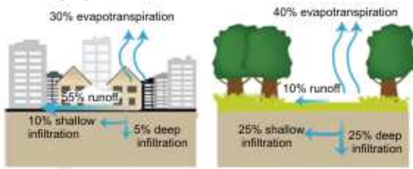
Fig.4. Evapotranspiration in urban areas (USEPA, 2008)
