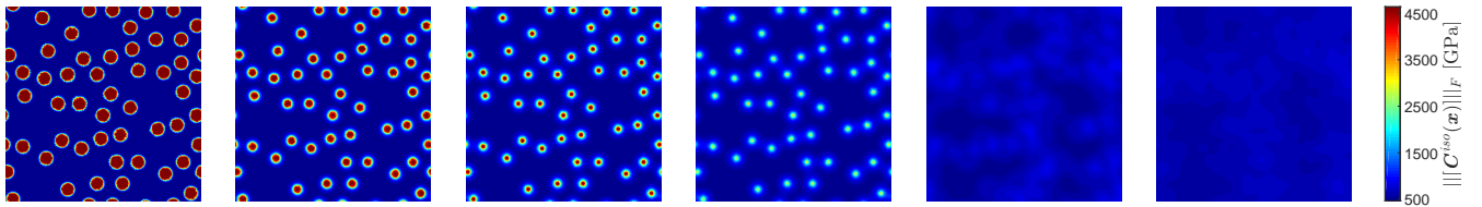
FIGURE 10 One realization of the random field \{|||C^{iso}(\mathbf{x})|||_F, \mathbf{x} \in \Omega\} for \tilde{R}/R \in \{0.2, 0.6, 0.8, 1, 2, 4\} (from left to right).
