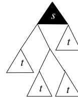
Fig. 1 A transitive tree-shift language. Let u denotes the tree pictured. If s denotes the black block and t the white one, s is a subtree of u rooted at \varepsilon , and t is a subtree of u rooted at any x \in X , where X is the complete prefix code \{00, 010, 011, 1\} .
