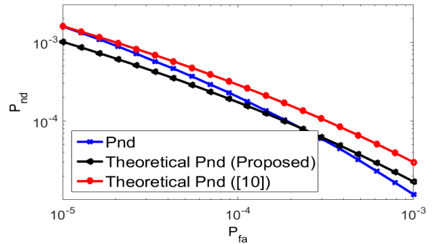
Fig. 4. Empirical and theoretical ROC curves for L=20 , \sigma^2 = 7/M
