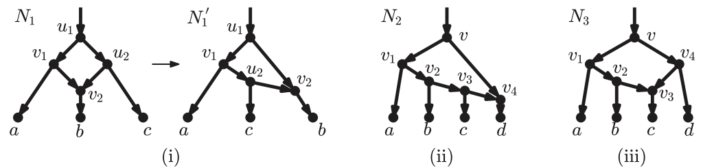
Fig 9. Reasons why the bound of Prop. 2 is not tight. (i) rNNI moves around different arcs may give the same network: the rNNI type-(1) move (u_1u_2, u_1v_1, v_1v_2 \rightarrow u_1v_2, u_1v_1, v_1u_2) and the rNNI type-(2) move (u_1u_2, u_2v_2, v_1v_2 \rightarrow u_1v_2, u_2v_2, v_1u_2) on N_1 both give the network N'_1 . (ii) Some of the moves drawn in Fig. 8 are not viable rNNI moves: no move of type BR around arc vv_4 of N_2 is allowed, because of the presence of a v_1 - v_3 path, which would cause the resulting network to contain a cycle. (iii) The bound of Prop. 2 is tight for some networks: the size of the rNNI neighborhood of network N_3 , equal to 12, coincides with the bound.
