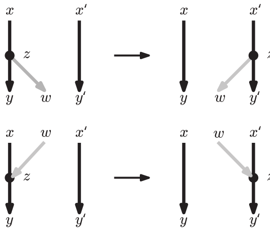
Fig 6. Illustration of rSPR moves.
