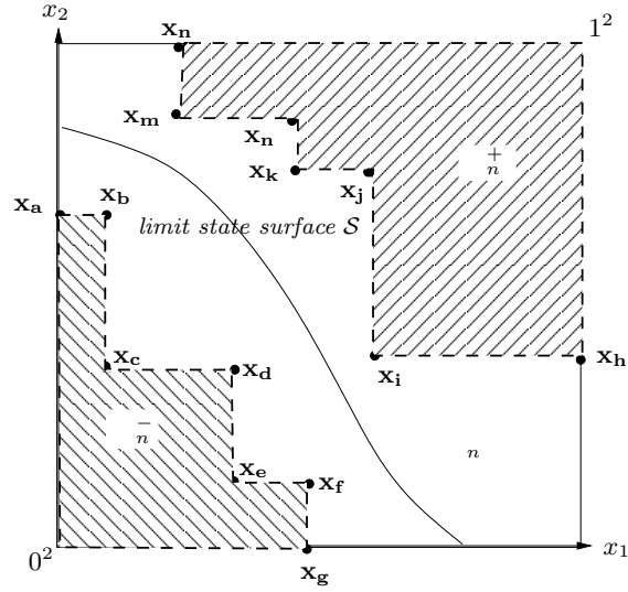
FIGURE 1. Two-dimensional dominated and non-dominated subspaces after n = 14 iterations. Points \{0^2, x_a, x_b, x_c, x_d, x_e, x_f, x_g\} have nonzero signatures and are vertices of \bar{\cdot}_n . Points \{x_h, x_i, x_j, x_k, x_l, x_m, x_n, 1^2\} have zero signatures and are vertices of \bar{\cdot}_n .
