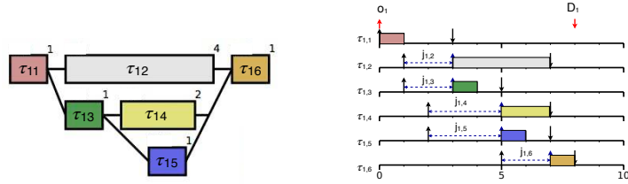
(a) A DAG task \tau_1 consists of 6 subtasks with parameters: D_1 = 8 , C_1 = 10 , L_1 = 6 .
