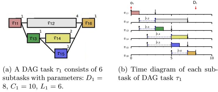
Fig. 1. Example of DAG model.
