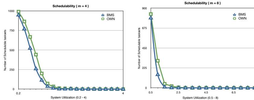
Fig. 6. Simulation results.
