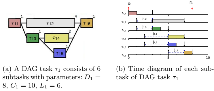
Fig. 1. Example of DAG model.
