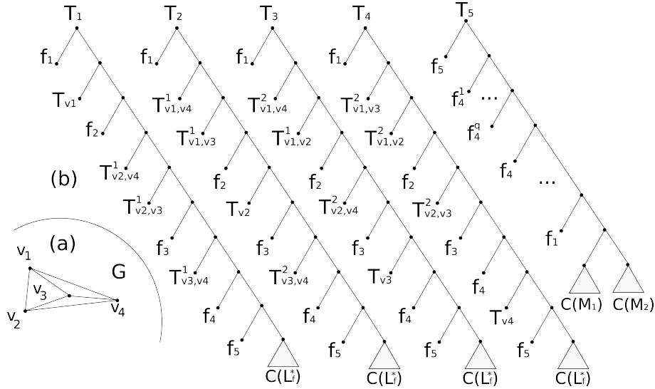
Figure 5: Gene trees T_1 to T_5 obtained from the cubic graph G where L_f = \langle f_5, f_4^1, \dots, f_4^q, \dots, f_1^1, \dots, f_1^q, f_1 \rangle and \forall 1 \leq i \leq 4, \lambda(v_i) = i . Each tree T_i , 1 \leq i \leq 4 , is obtained by inserting tree T_{v_j} , T_{j,h}^x in the comb graph C(\langle f_1, \dots, f_5 \rangle) . Notice that T_5 contains a comb graph C(\langle f_5, \dots, f_1 \rangle) .
