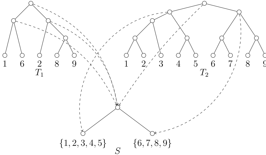
Figure 2: A set \mathcal{F} = (T_1, T_2) of gene trees and the species tree S which is a bipartition ( \{1, 2, 3, 4, 5\}, \{6, 7, 8, 9\} ). For sake of clarity, we have labelled the leaves of T_1 and T_2 with the species of S . The only node with a pre-duplication is the root of T_1 , since this node and its two children are mapped by \mathcal{M} (via the dashed lines) to the root of S . Still for sake of clarity, the mapping is not drawn for all nodes of T_1 and T_2 .
