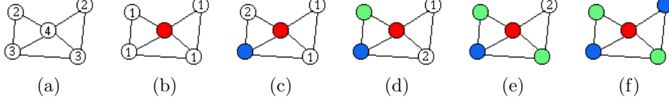
FIG. 2.2. Coloring a graph using the DSAT algorithm [55]. (a) Sort nodes by decreasing degree. Initial labeling DSAT equal to node degrees. (b) Choose a node with maximum DSAT. Assign color number 1. Update DSAT: For each non-colored node v , if at least one neighbor of v is colored, DSAT(v) equals the number of different colors used in the neighborhood of v . (c) Choose a non-colored node of maximum DSAT. In case of conflict, choose a node of maximum degree. Assign the smallest possible color. Update DSAT. (d,e,f) Repeat the procedure in (c) until all nodes are colored.
