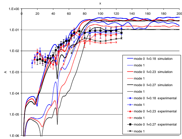
Figure 8. Influence of the forcing frequency on the evolution of the temperature fluctuations along the channel: experimental and numerical results. \epsilon = 2 , d = 0.14 .
