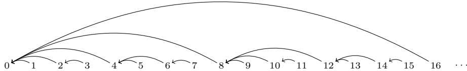
Figure 4: Graph of the flip function
