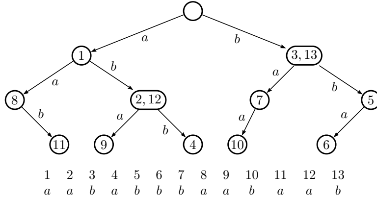
Figure 2: Position heap for string aababbbaabaab . Double nodes store pairs of positions.
