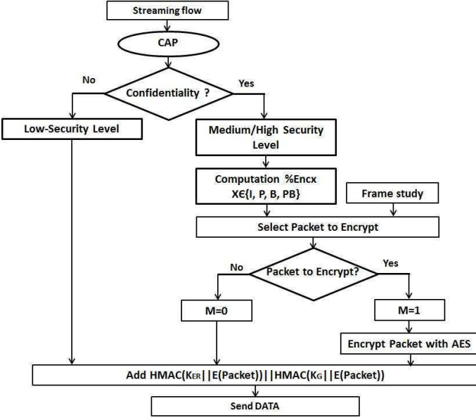
Fig. 1. Flowchart of EDES at the Sender node
