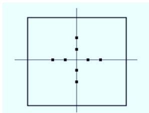
Fig. 3 : Illustration of the position of JPEG spots observed at the frequency of 1/8 and the first harmonic.
