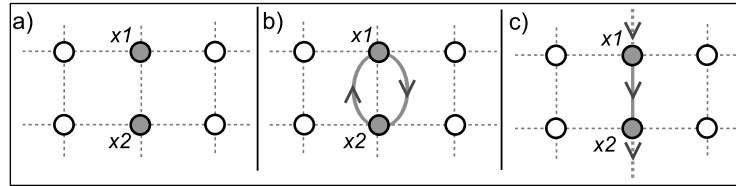
Fig. 3. Loops in toric spaces - In the toric space \mathbb{Z}_3 \times \mathbb{Z}_2 (see a), the sequence of points (\mathbf{x}_1, \mathbf{x}_2, \mathbf{x}_1) can be interpreted in two different ways: b) and c).
