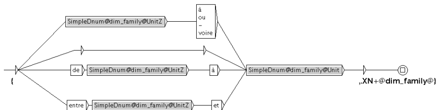
Fig. 5. parameterized DnumUnit
