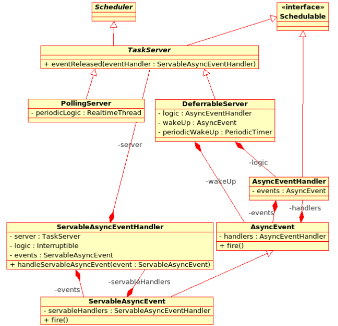
Figure 2: Classes to implement the server policies
