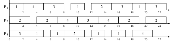
Figure 2. Scheduling at job boundaries.
