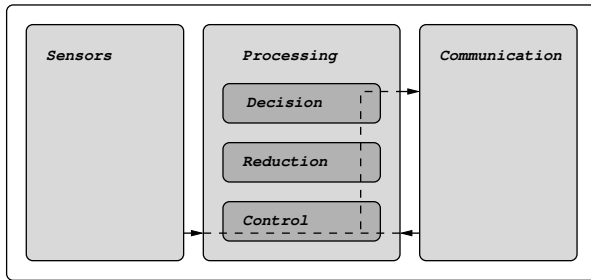
Figure 1. A model for a sensor embedded system
