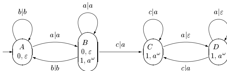
Fig. 6. Determinization of the transducer of Fig. 4
