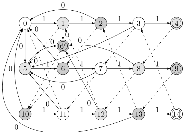
Fig. 5. A presentation of S_{U,T}^{\sigma} for S = \text{MTR}(3) , T = 3 , U = \{1\} . It is obtained by Algorithm PERIODIC-AUTOMATON on the input tries accepting the sets \mathcal{G}^{(0)} = \{1111\} , \mathcal{G}^{(1)} = \{0, 1111\} , \mathcal{G}^{(2)} = \{1111\} . States in phase 0, 1, and 2 are colored in white, light gray, and gray respectively.
