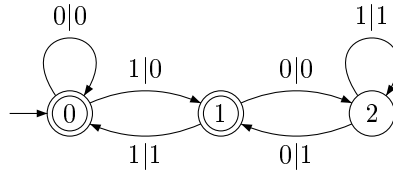
Figure 1: Sequential Büchi transducer of Example 1
