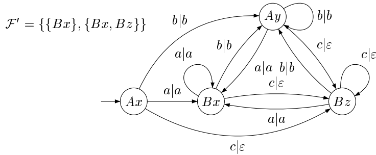
Figure 8: Transducer \mathcal{S}' of Example 17
