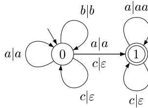
Figure 5: Transducer \mathcal{T} of Example 17
